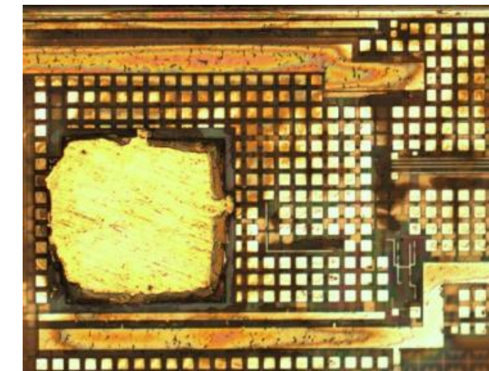
Cover layer
