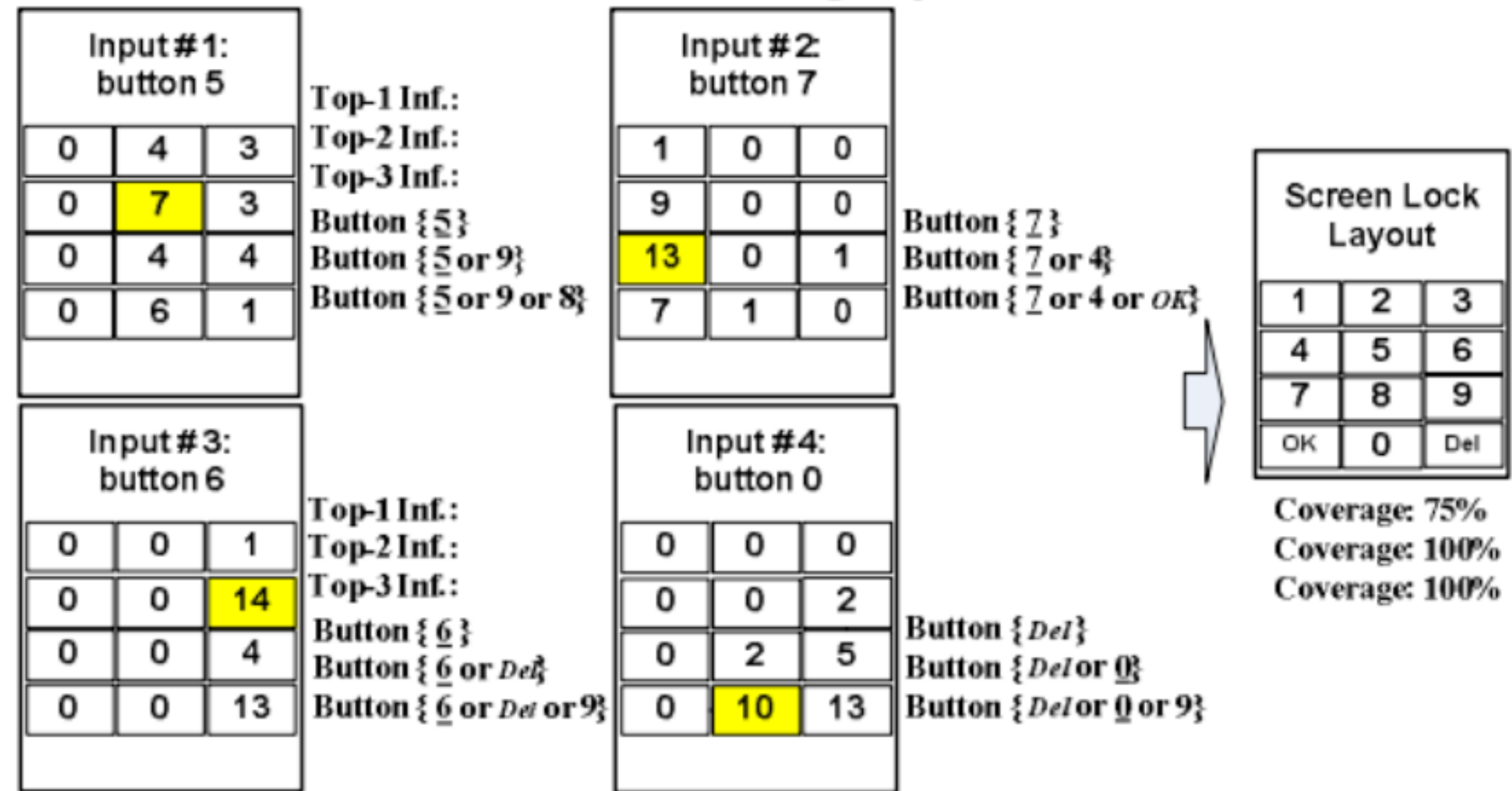
Distribution of inferred labels after entering the passwords "5 7 6 0" for 32 rounds
